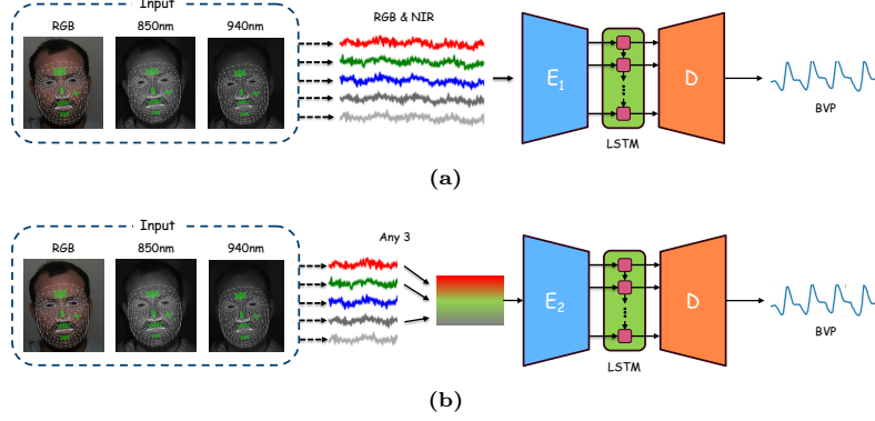
Fig. 4: Encoder-decoder model to test different combinations of R, G, B, IR(850nm), and IR(940nm) channels for rPPG information retrieval. Two models were developed: (a) takes all five channels as input simultaneously; and (b) takes any three channels.
